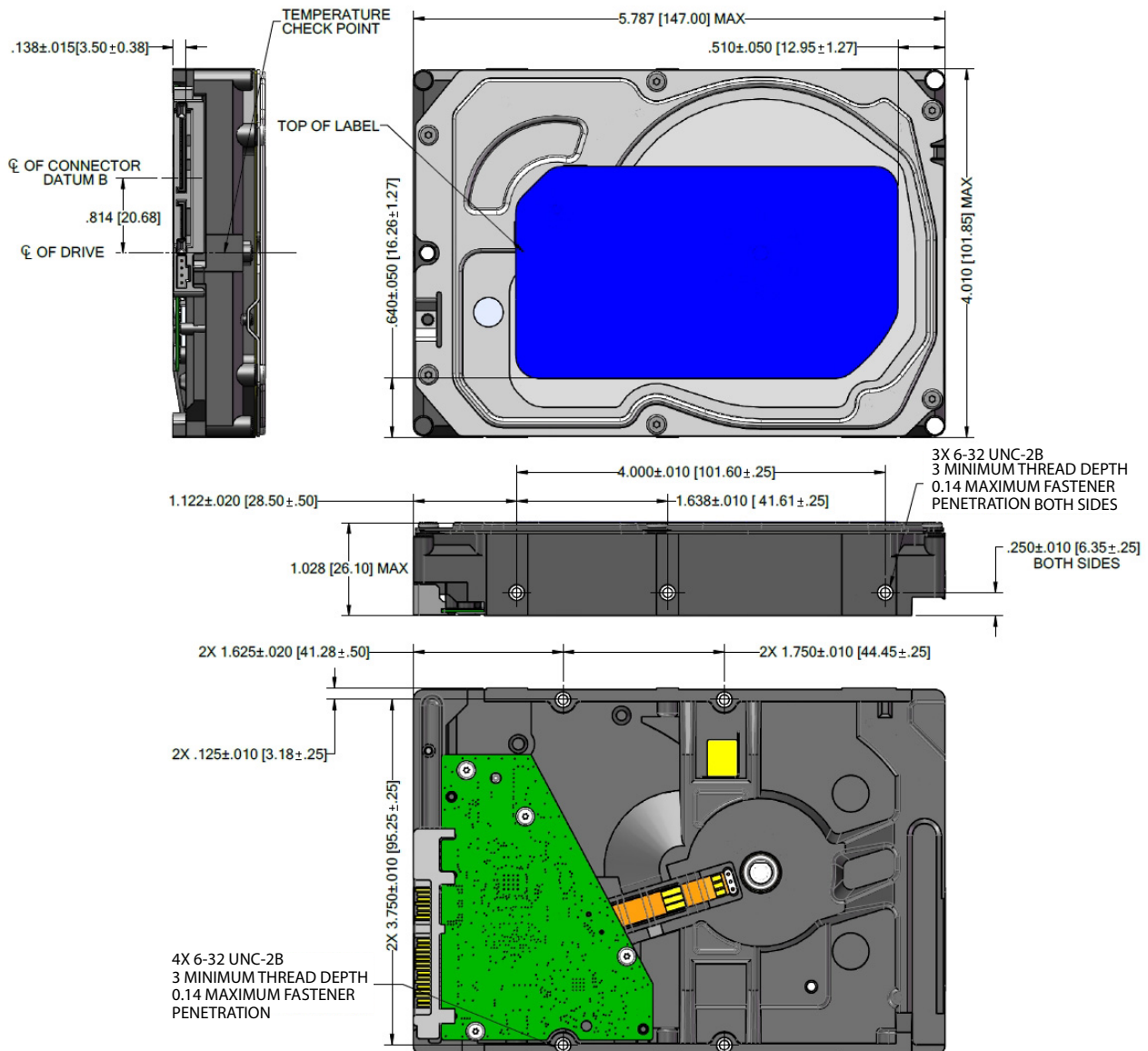
Figure 4 Mounting dimensions (4-disk models)
