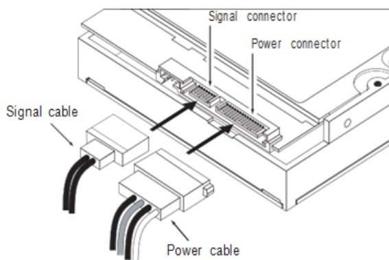
Figure 3 Attaching SATA cabling
