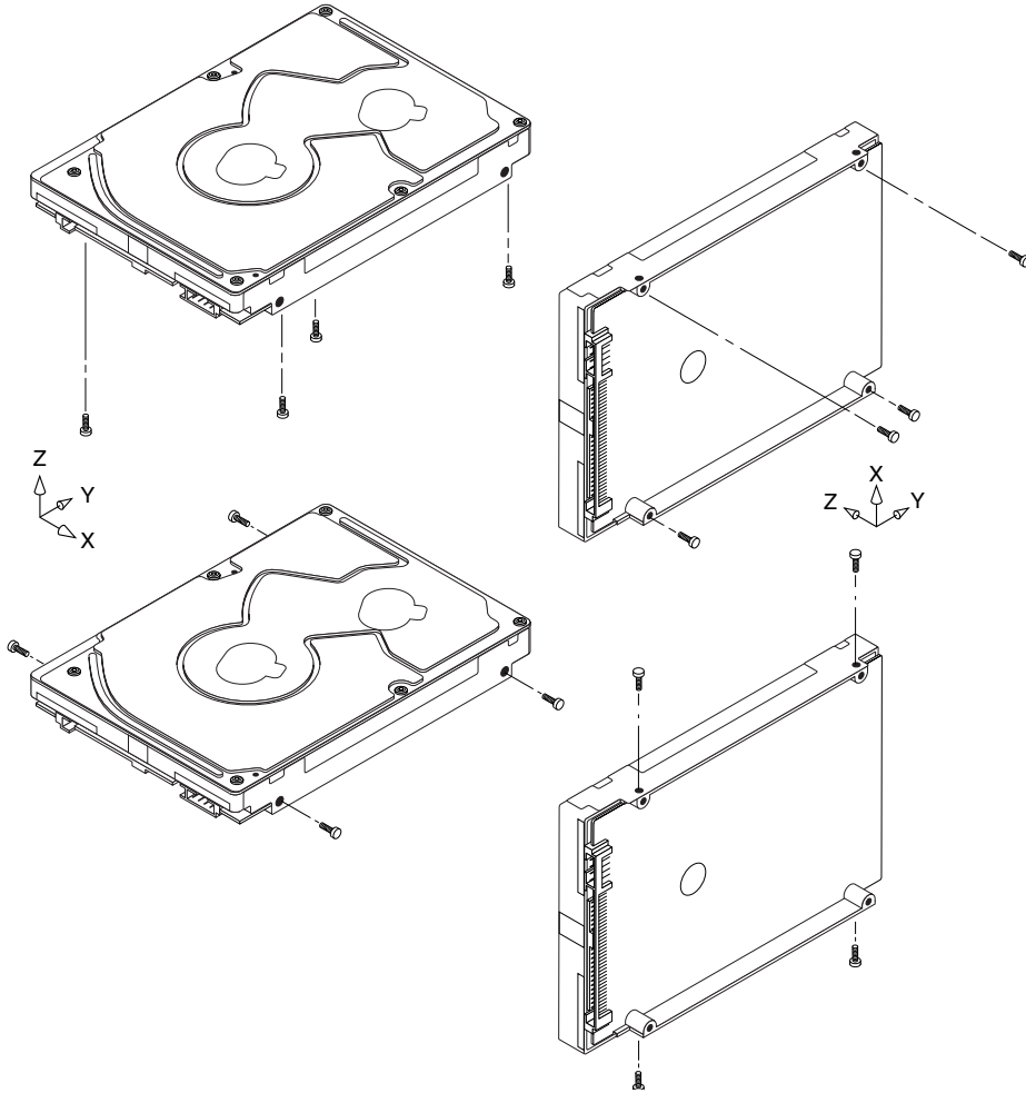
Figure 14. Recommended mounting
