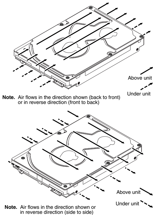
Figure 18. Air flow
