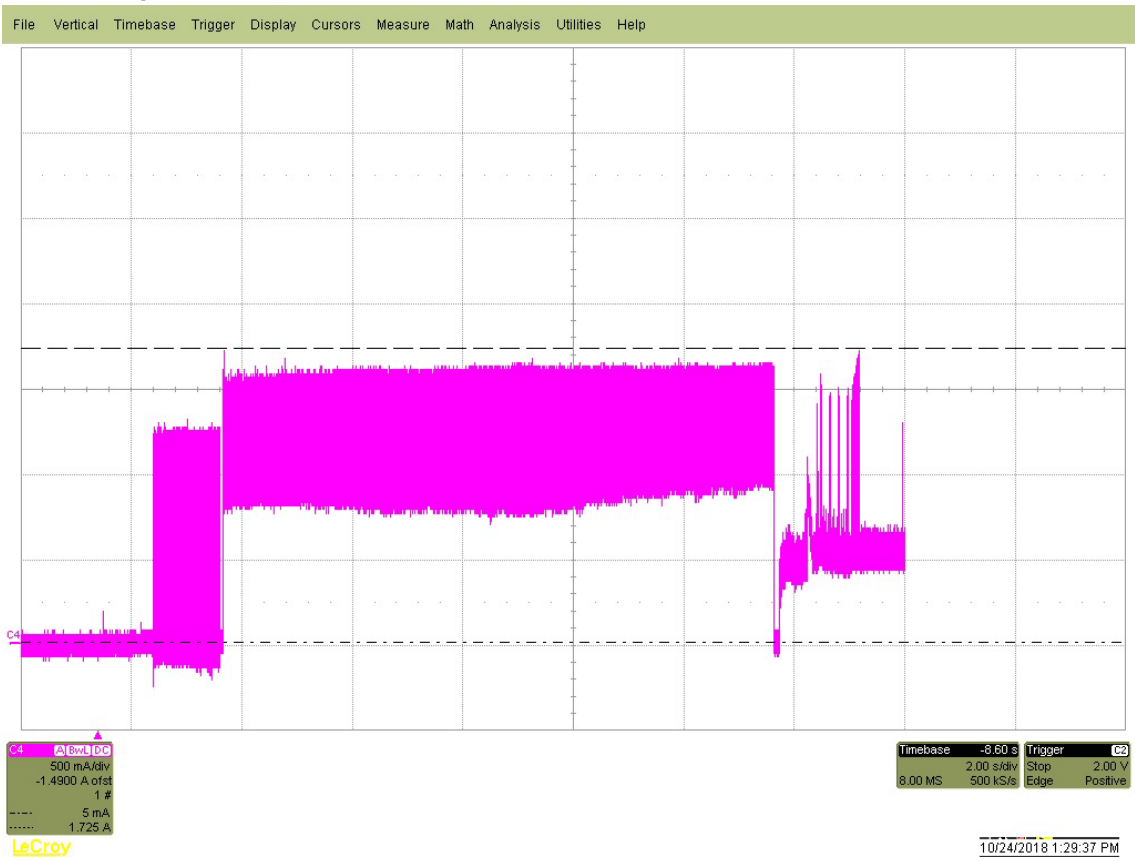
Figure 1. 8TB & 6TB Typical 12V startup and operation current profile
